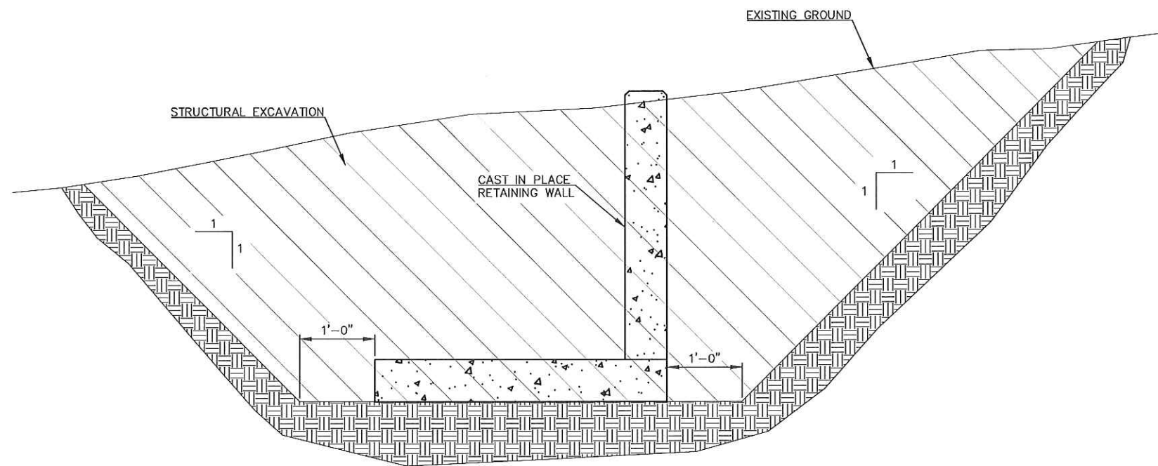
LIMITS OF STRUCTURAL EXCAVATION FOR RETAINING WALL
