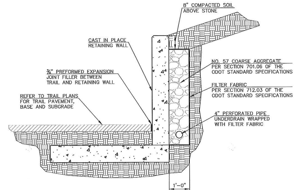
RETAINING WALL BACKFILL
