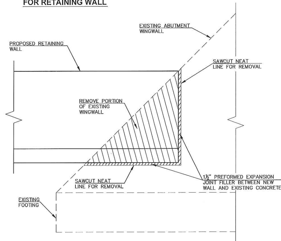
RETAINING WALL TO WINGWALL DETAIL
